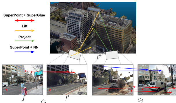
Figure 8: Illustration of the Lift-and-Project optimization.
