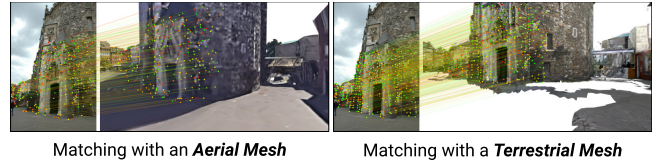
Figure 9: Aerial meshes lack texture comparing to terrestrial meshes, resulting in less matches.
