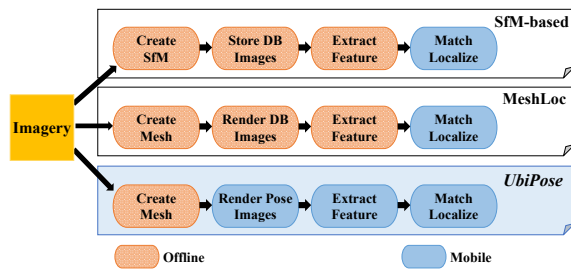
Figure 5: Different approaches to AR pose tracking at scale.
